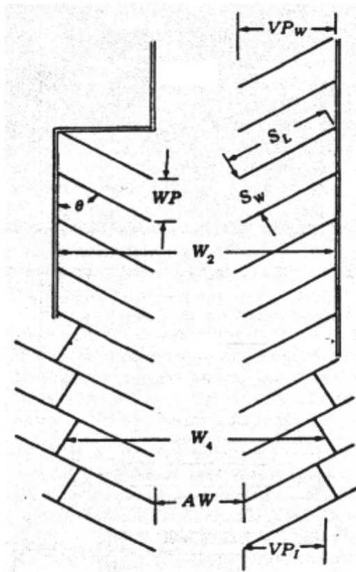
Figure 9.1.1 Parking Dimensional Layout Diagram
